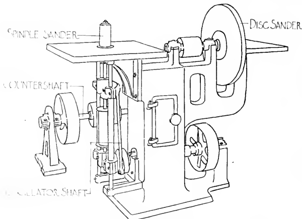
FIG. 206. SPINDLE AND DISC SANDER.
